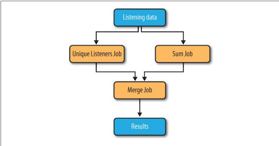
Figure 14-2. TrackStats jobs
