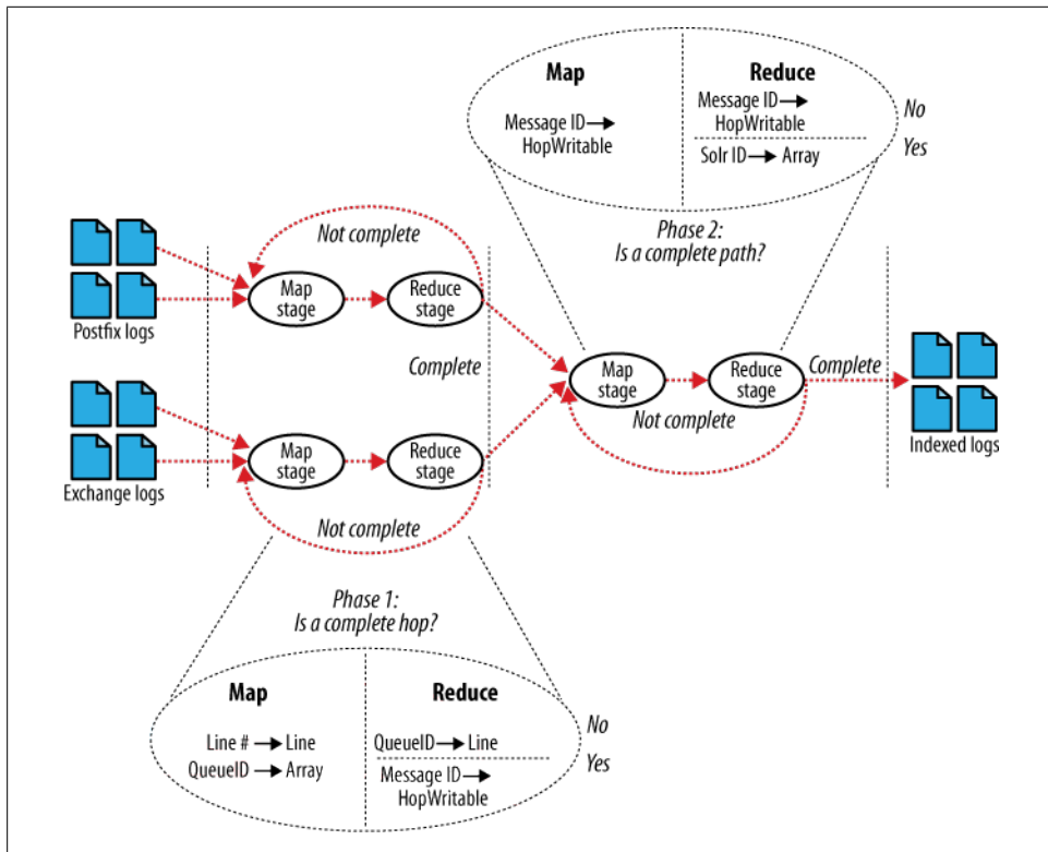
Figure 14-9. MapReduce chain
